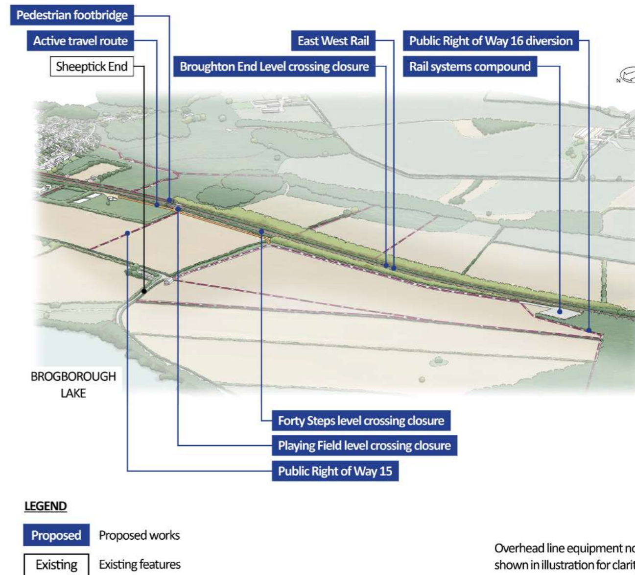
Figure 44: An indicative aerial illustration of how we propose to use active travel routes to mitigate level crossing closures
