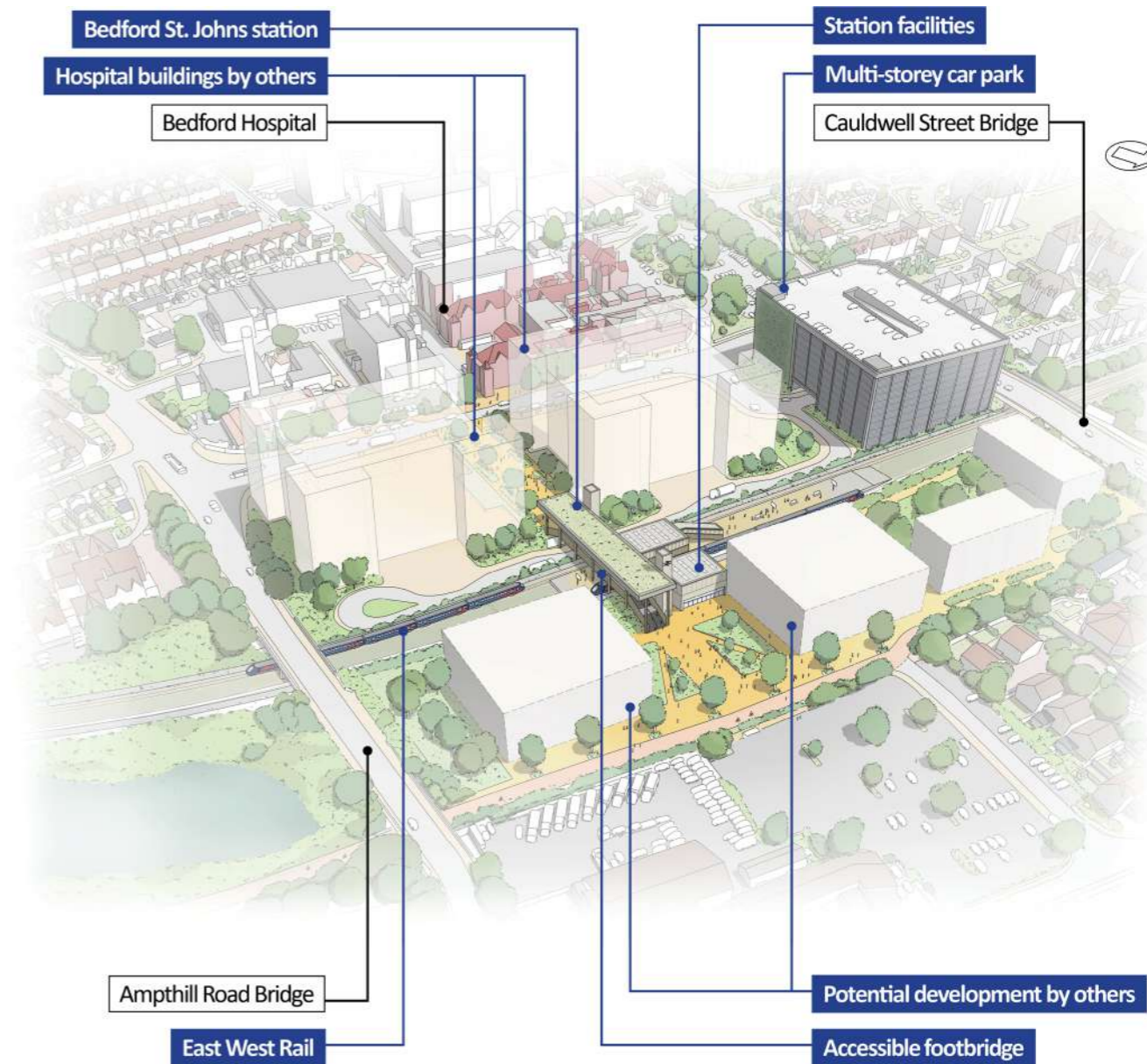
Figure 51: An indicative aerial illustration of the relocated Bedford St Johns station
