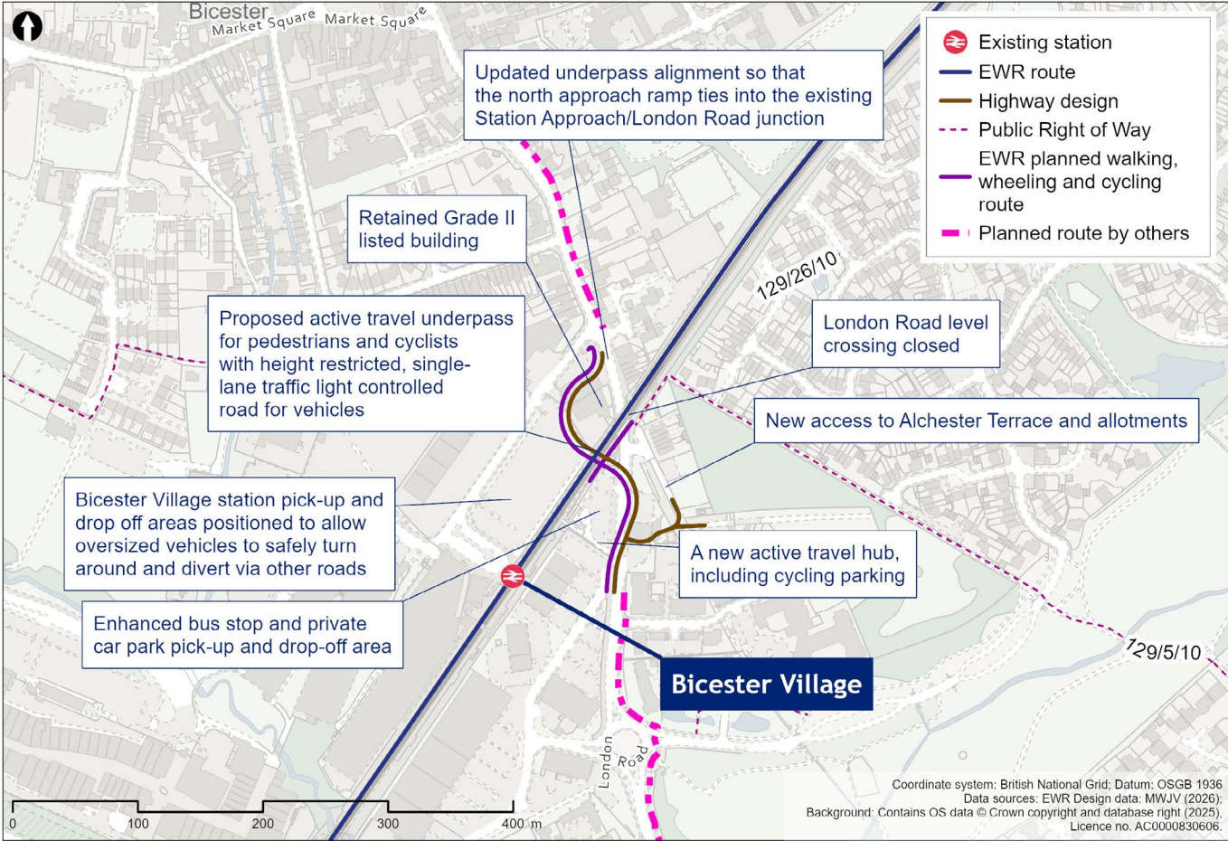
Figure 21: Map of the underpass at London Road, Bicester
