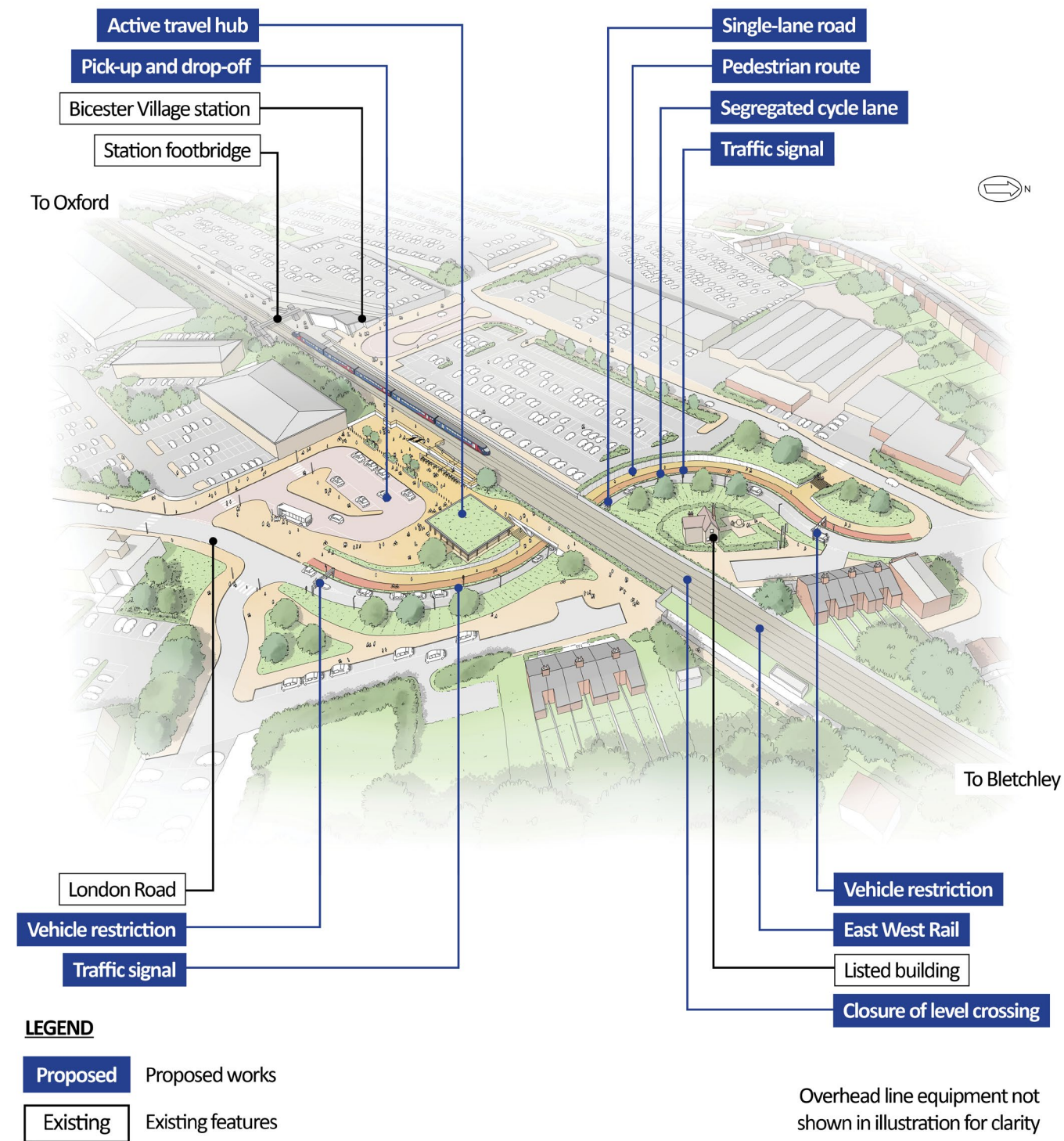
Figure 22: An indicative aerial illustration of the underpass at London Road, Bicester
