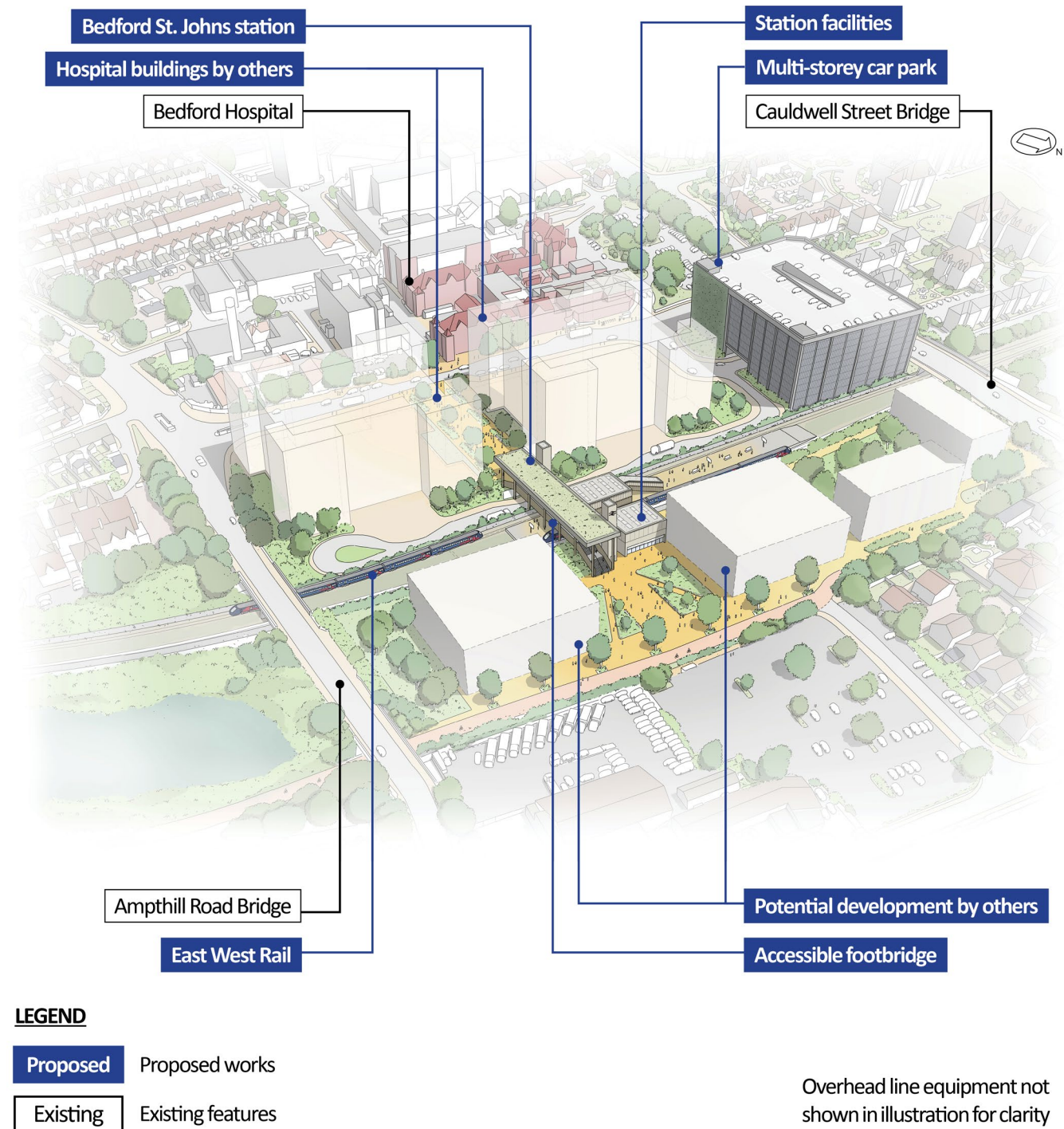
Figure 51: An indicative aerial illustration of the relocated Bedford St Johns station
