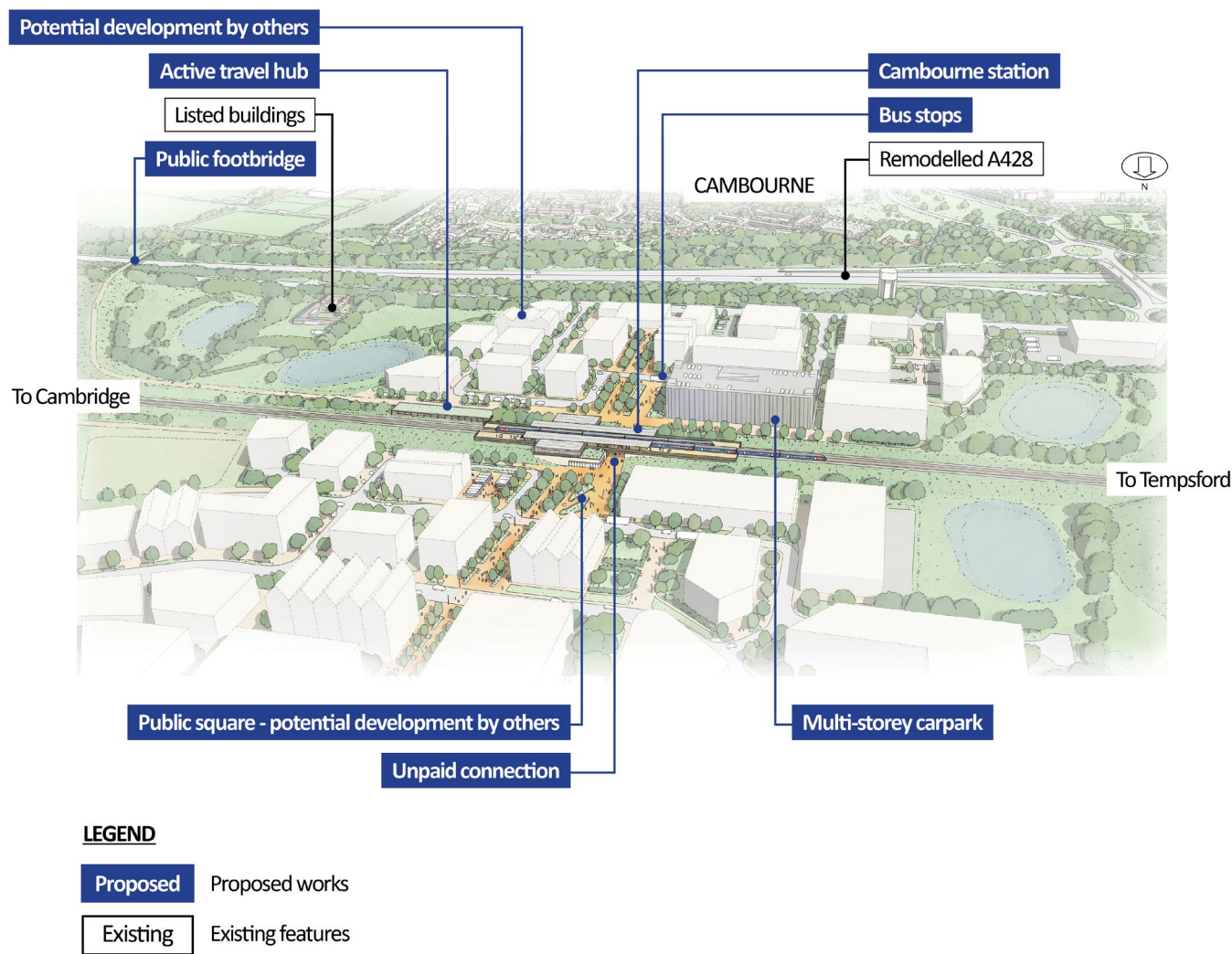
Figure 77: An indicative aerial illustration of Cambourne station
