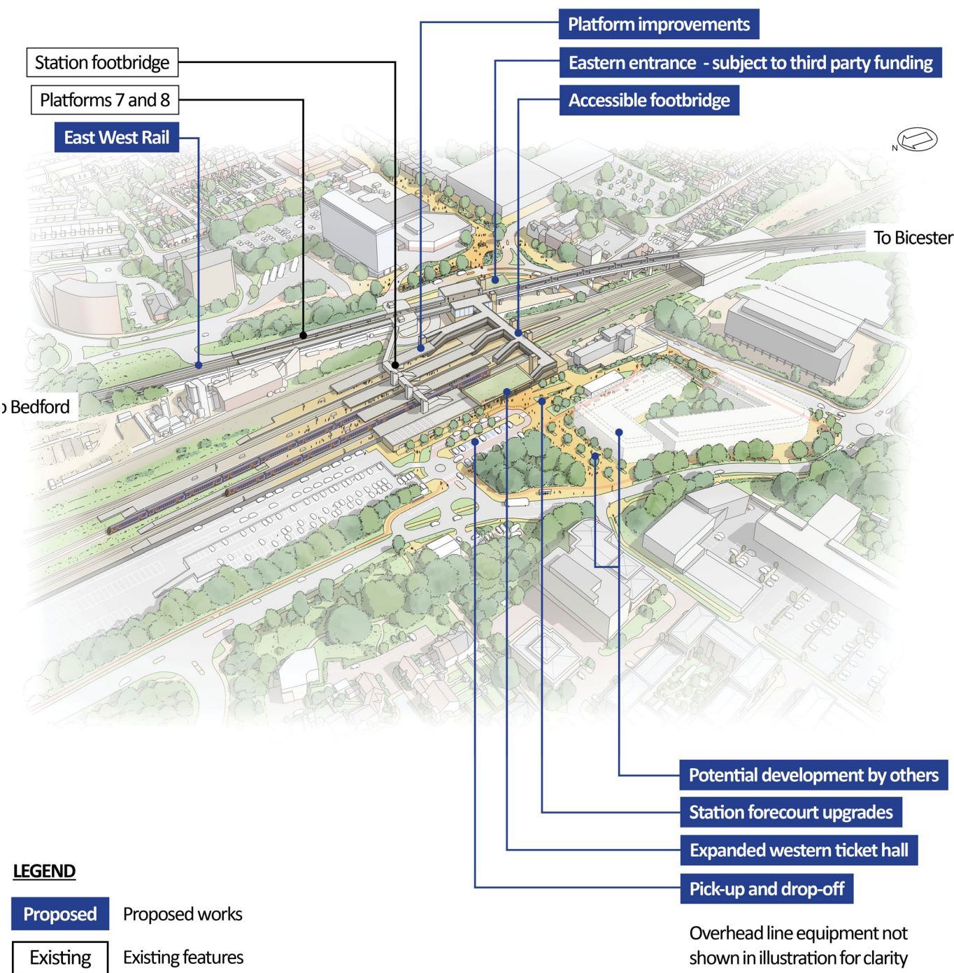
Figure 31: An indicative aerial illustration of Bletchley station
