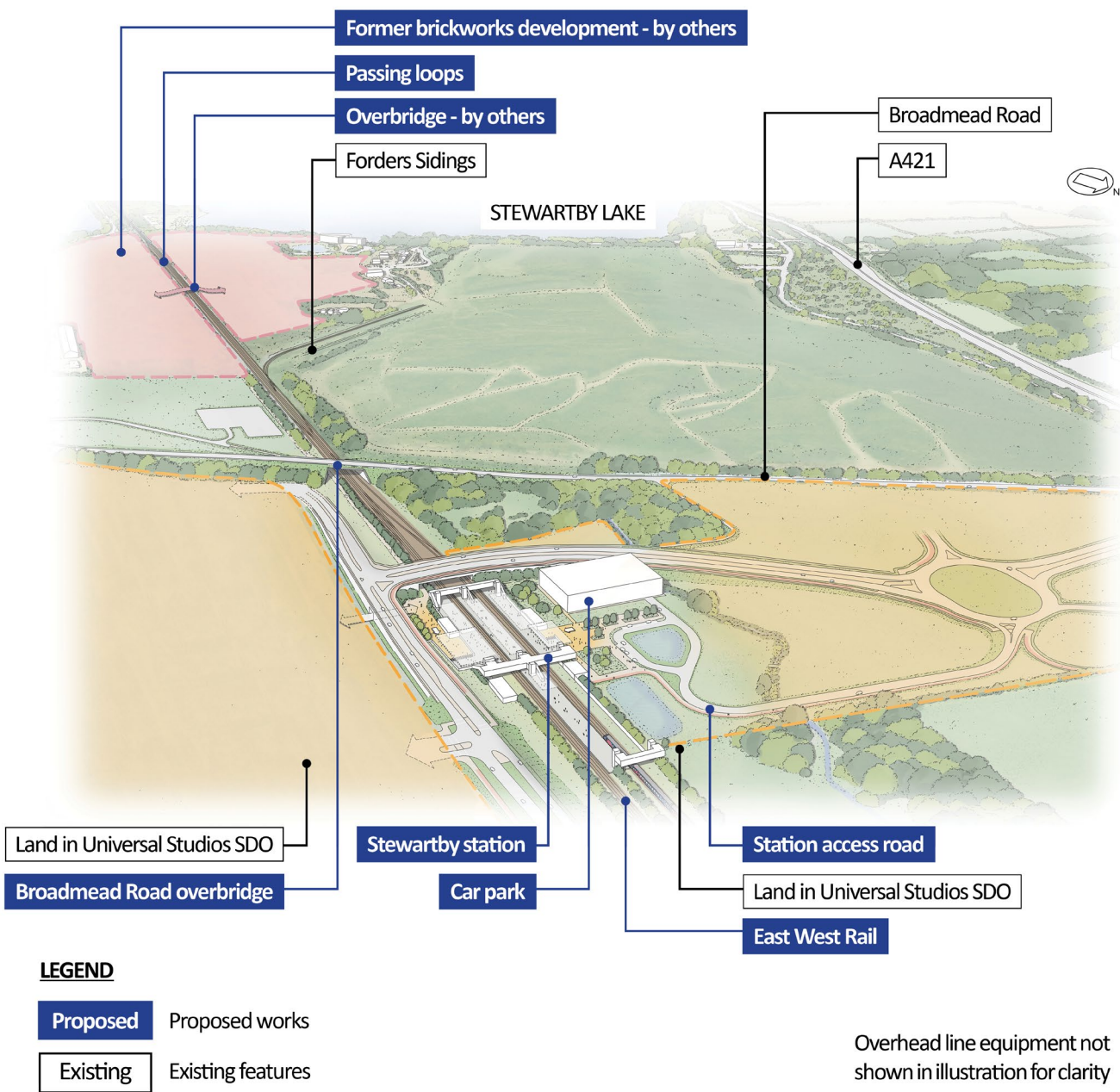
Figure 46: An indicative aerial illustration of the new Stewartby station including loops south of the station. Detail of proposals within the Entertainment Resort Complex Special Development Order boundary is subject to ongoing discussions.
