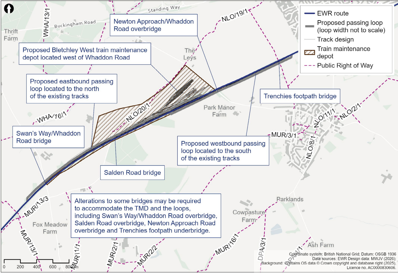
Figure 26: Map of the Bletchley West train maintenance depot and passing loops
