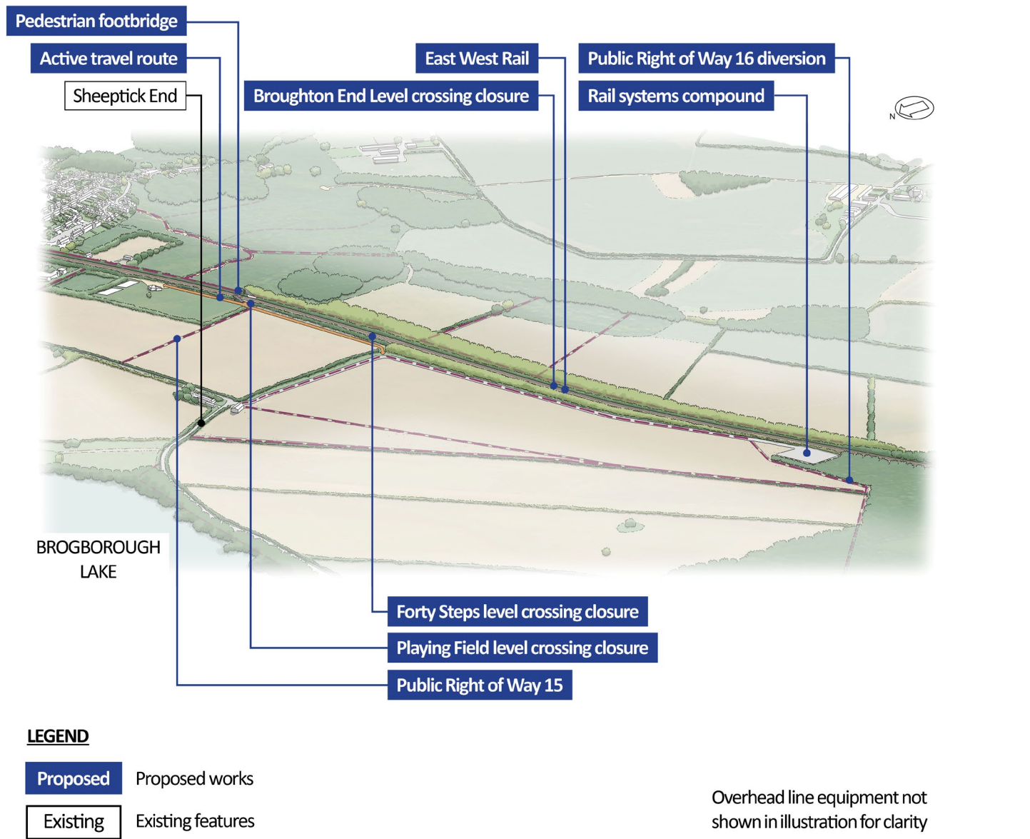
Figure 44: An indicative aerial illustration of how we propose to use active travel routes to mitigate level crossing closures
